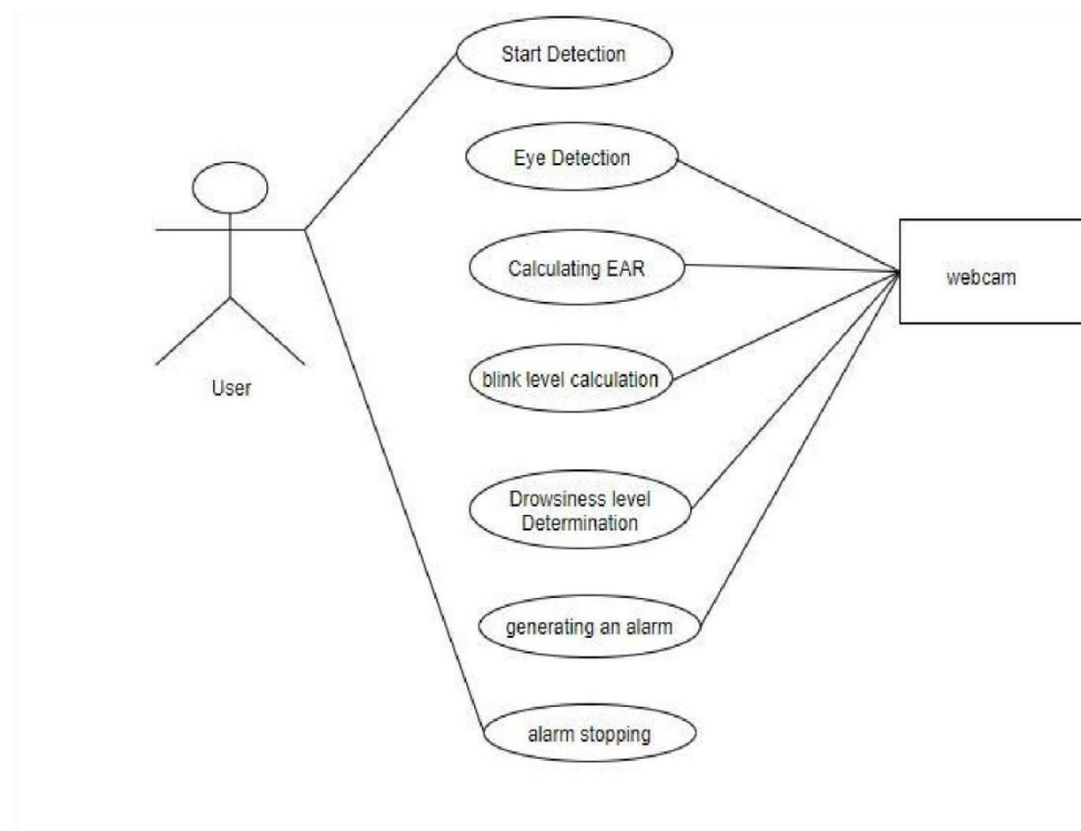
Fig 4.3.1 Use Case Diagram for Proposed System
