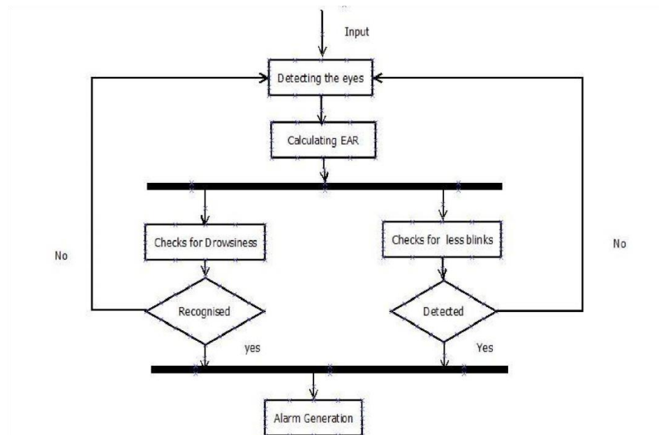
Fig 4.4.3 Data Flow Diagram of the system
