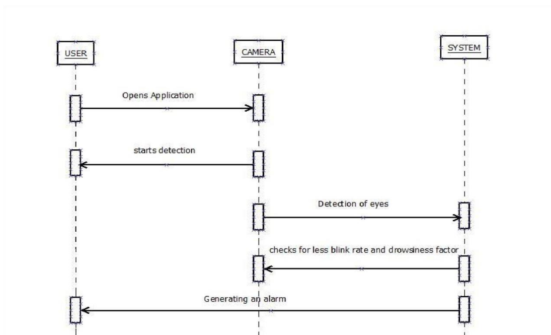
Fig 4.3.2 Sequence Diagram of Proposed System
